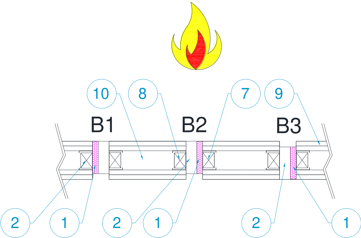
Figure 5 – Cross-section of specimens B1 to B3
