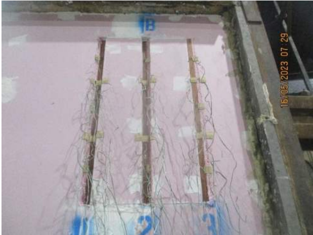
Specimens B1-B3
