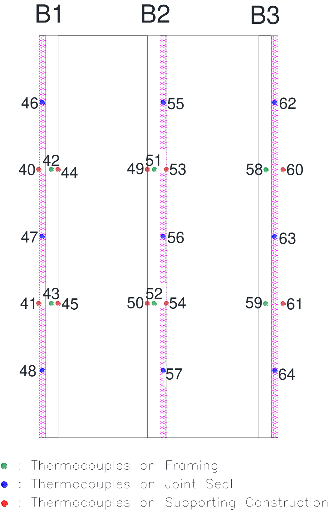
Figure 4 – Unexposed face elevation of the specimens B1 to B3 with thermocouple locations
